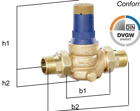
DN 15 - DN 32 (DRV 403-6)
